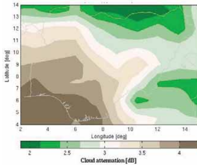
Fig. 9: Contour Map of Cloud attenuation for V downlink (40GHz) from NigComsat-1 at 0.01% unavailability
