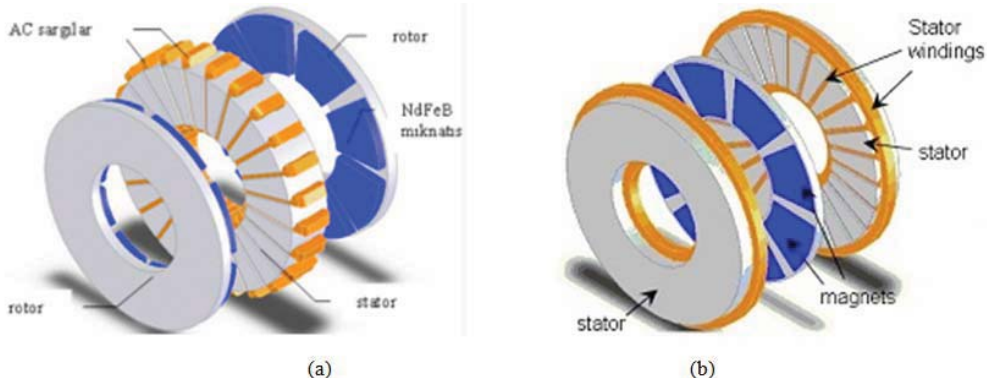
Fig. 1: Axial flux non-slotted (a) one-stator-two-rotor TORUS-NS type (Gholamian, S.A., et al , 2008) (b) two-stator-one-rotor AFIR-NS type (Gholamian, S.A., 2008)
