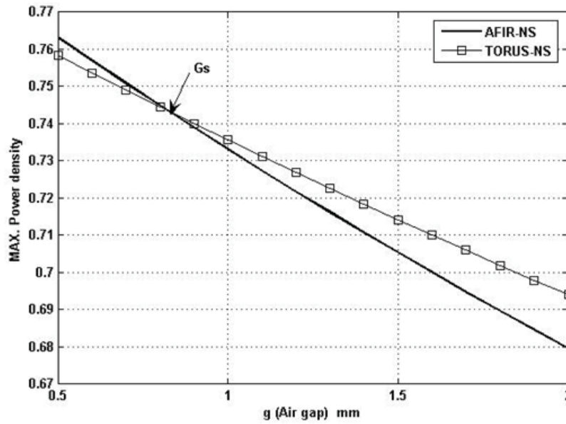
Fig. 6: Maximum power density AFIR-NS and TORUS-NS vs. air-gap length
