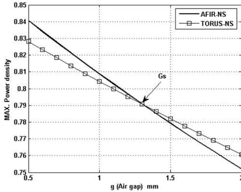
Fig. 5: Maximum power density AFIR-NS and TORUS-NS vs. air-gap length
