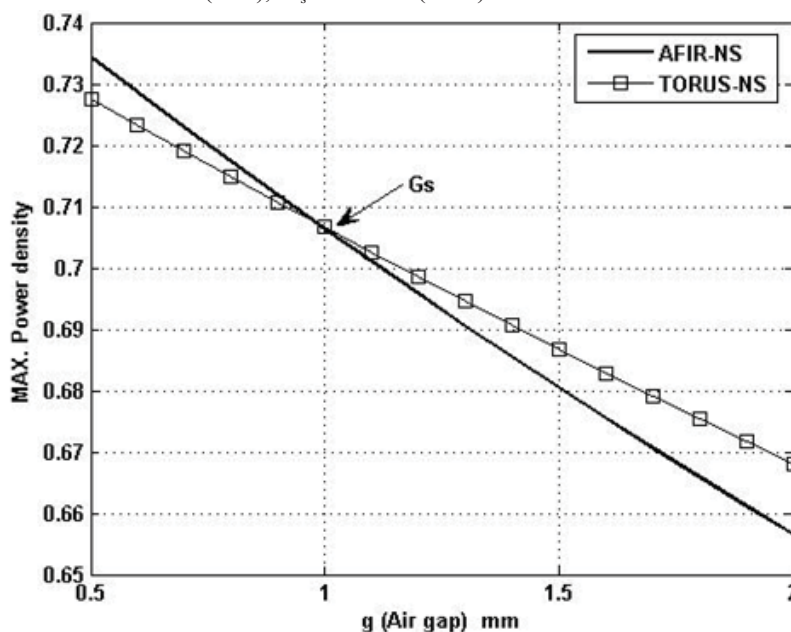
Fig. 4: Maximum power density AFIR-S and TORUS-NS vs. air-gap length
