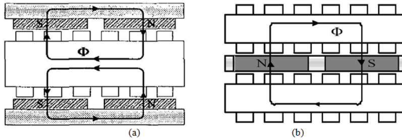
Fig. 2: One pole pair of the (a) TORUS-NS (Gholamian, S.A., et al , 2008) (b) AFIR-NS (Gholamian, S.A., 2008)
