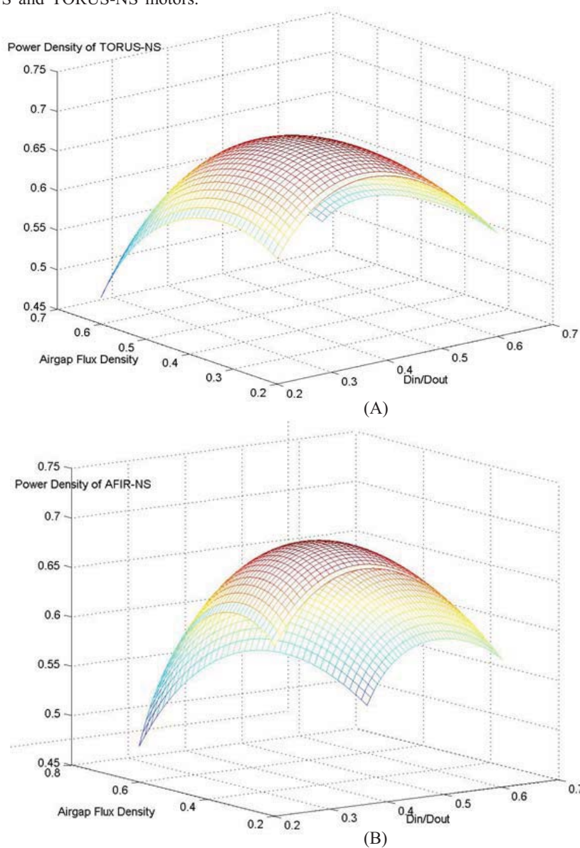
Fig. 3: Power density vs. air-gap flux density and diameter ratio for A=20000 (A/m), g=1 (mm), J_s=6000000 (A/m 2 )
