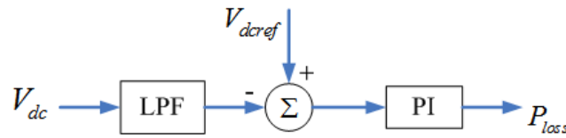
Fig. 3: DC link voltage control block diagram.
