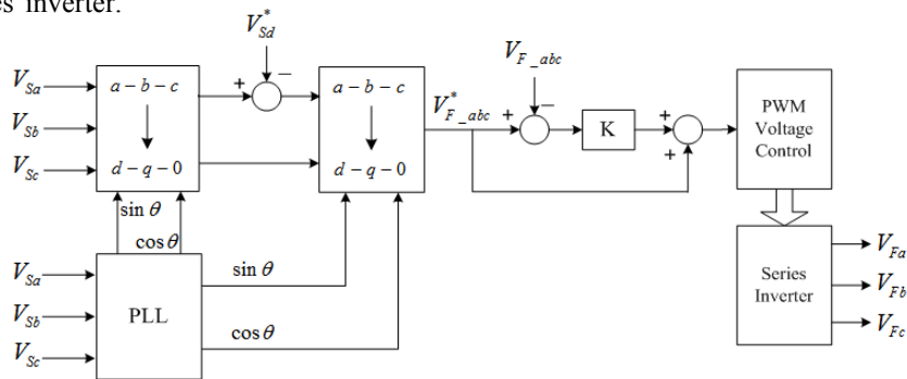
Fig. 4: Series inverter control block diagram.
