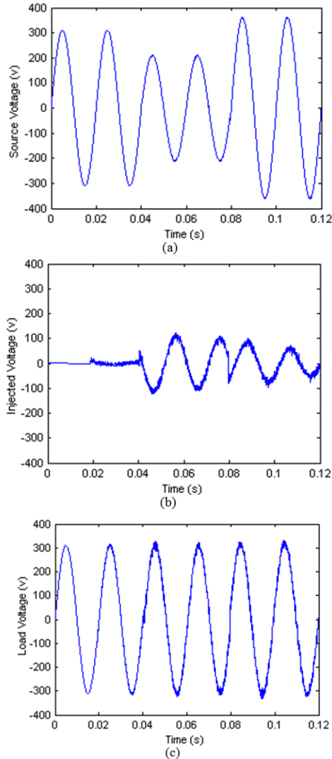
Fig. 10: (a) Source voltage, (b) Injected voltage, (c) load voltage, before and after compensation.
