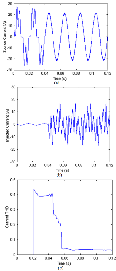
Fig. 9: (a) Source current, (b) Injected current, (c) source current THD, before and after compensation.
