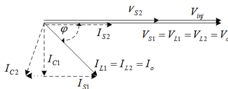
Fig. 5: Phasor diagram of shunt and series inverters loading.
