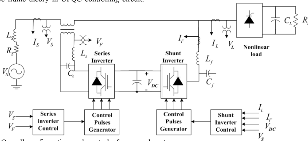
Fig. 1: Overall configuration and control of proposed system.
