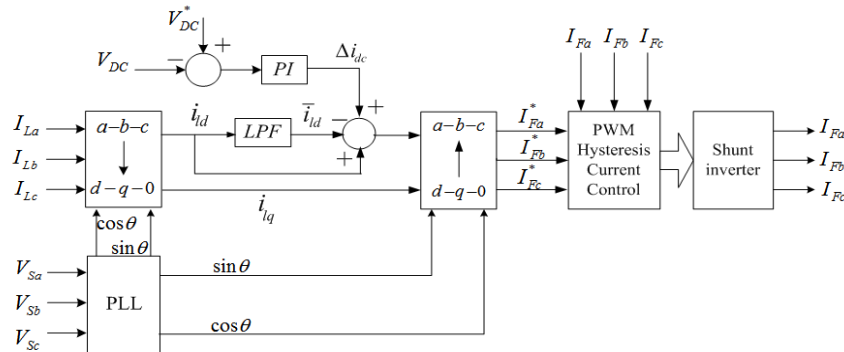
Fig. 2: Shunt inverter control block diagram.
