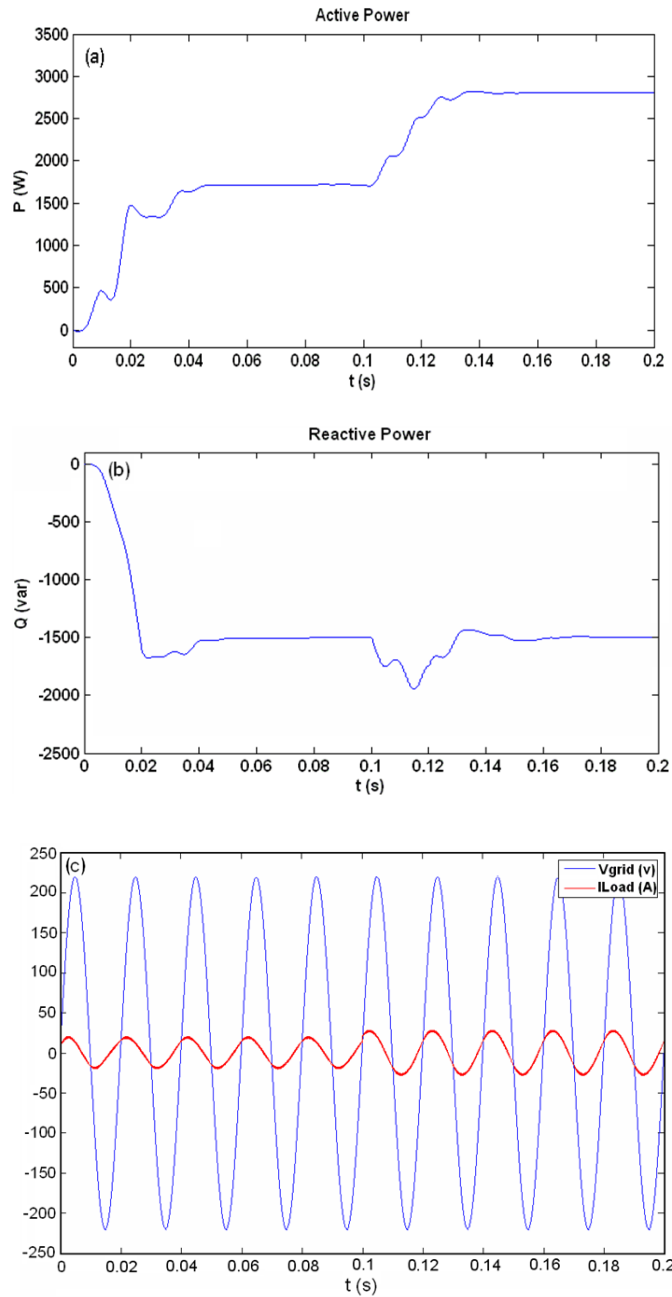
Fig. 7: System simulation results for sun radiation variation with applying MPPT and for and Q_{ref} = -1500\text{var} .
