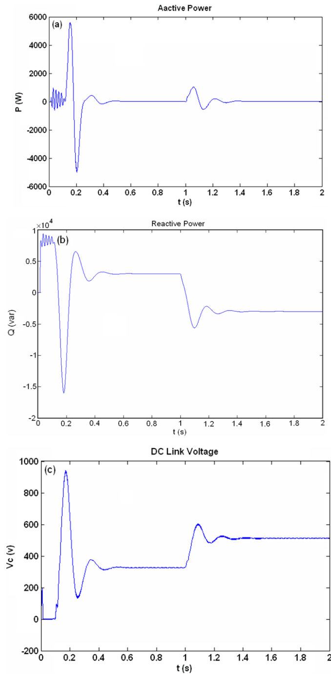
Fig. 8: System simulation results for night mode. a) active power, b) reactive power, c) DC link voltage.
