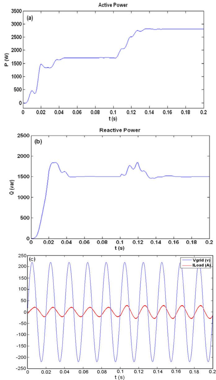
Fig. 6: System simulation results for sun radiation variation with applying MPPT and Q_{ref}=1500var .
