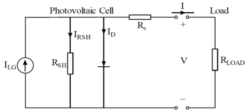
Fig. 1: Equivalent circuit of PV.
