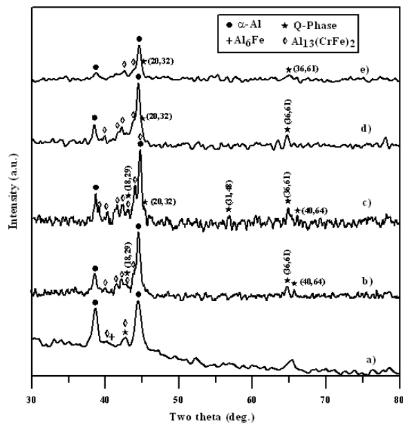
Fig. 4: XRD patterns for 40 hs mechanically alloyed "Al 86 Cr 8 Fe 6 " annealed at 360 C for: a) as milled, b) 10 hs, c) 30 hs, d) 50 hs, e) 70 hs.
