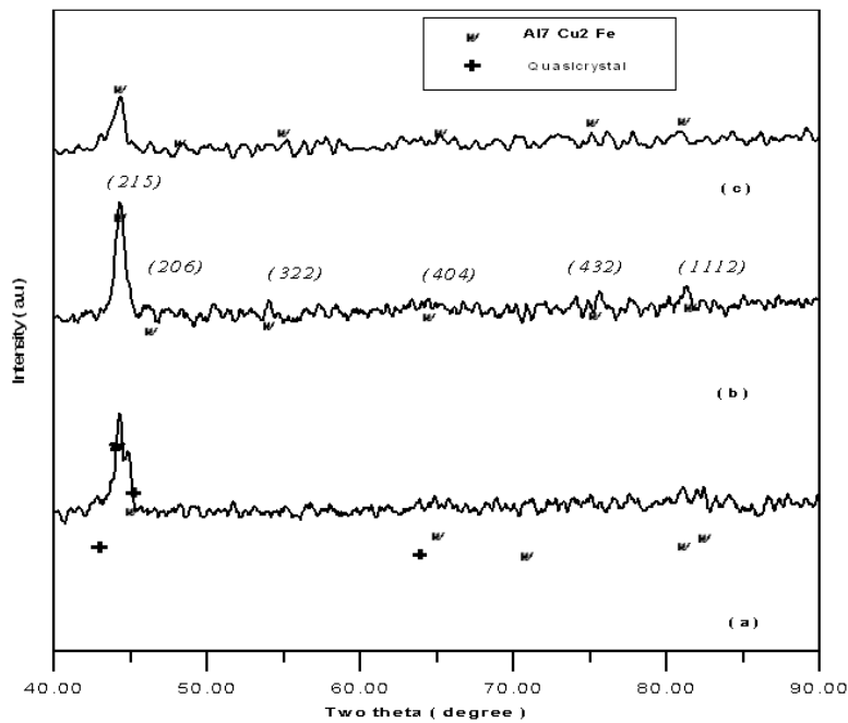
Fig. 13: XRD patterns of "Al 62.5 Cu 25 Fe 12.5 " milled for 30 hs. followed by annealing for 1 min. at a) 450 C, b) 500 C, and c) 600 C.
