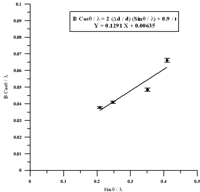
Fig. 2: Williamson-Hall plot for 40 hs milled powder for "Al 86 Cr 8 Fe 6 ".
