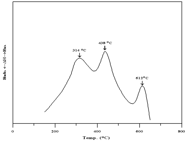
Fig. 3: DTA curve for 40 hs milled powder for "Al 86 Cr 8 Fe 6 ".
