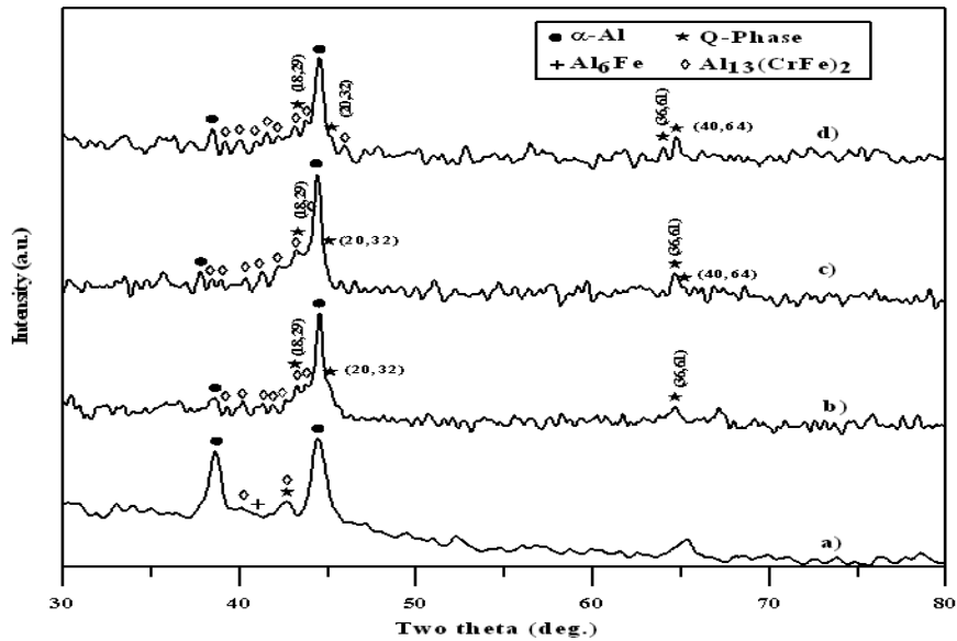
Fig. 5: XRD Patterns for 40 hs mechanically alloyed " \text{Al}_{86}\text{Cr}_8\text{Fe}_6 " annealed at 500 C for: a) as milled, b) 5 hs, c) 10 hs, d) 15 hs.
