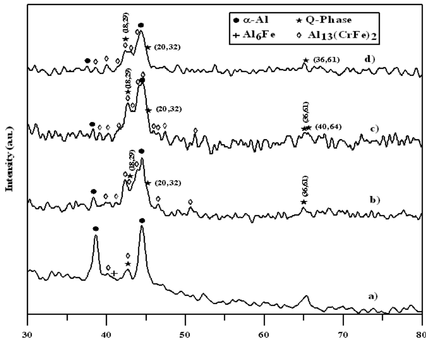
Fig. 6: XRD patterns for 40 hs mechanically alloyed " \text{Al}_{86}\text{Cr}_8\text{Fe}_6 " annealed at 650 C for: a) as milled, b) 5 hs, c) 10 hs, d) 15 hs.
