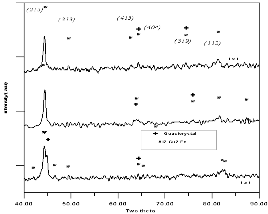
Fig. 12: XRD patterns of " \text{Al}_{62.5}\text{Cu}_{25}\text{Fe}_{12.5} " milled for 20 hs. followed by annealing for 1 min. at 450 C, 500 C, and 600 C respectively in upward way.
