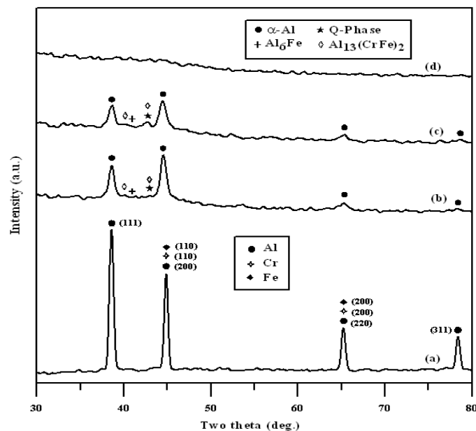
Fig. 1: XRD patterns of mechanically alloyed " \text{Al}_{86}\text{Cr}_8\text{Fe}_6 " for: a) 0 h b) 30 hs c) 40 hs d) 150 hs.
