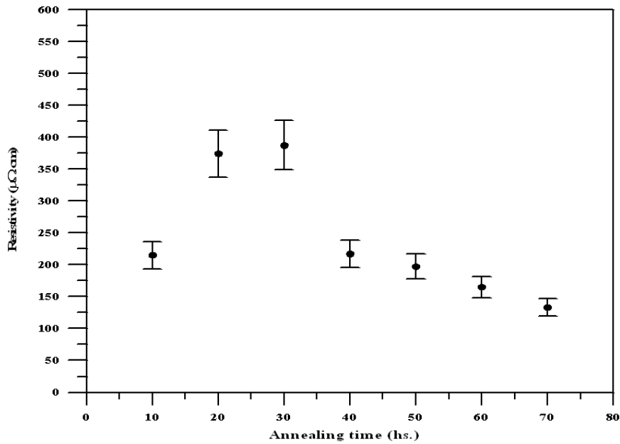
Fig. 7: Resistivity changes with the annealing time for 40 hs. Milled powder " Al_{86}Cr_8Fe_6 " annealed at 350 C.
