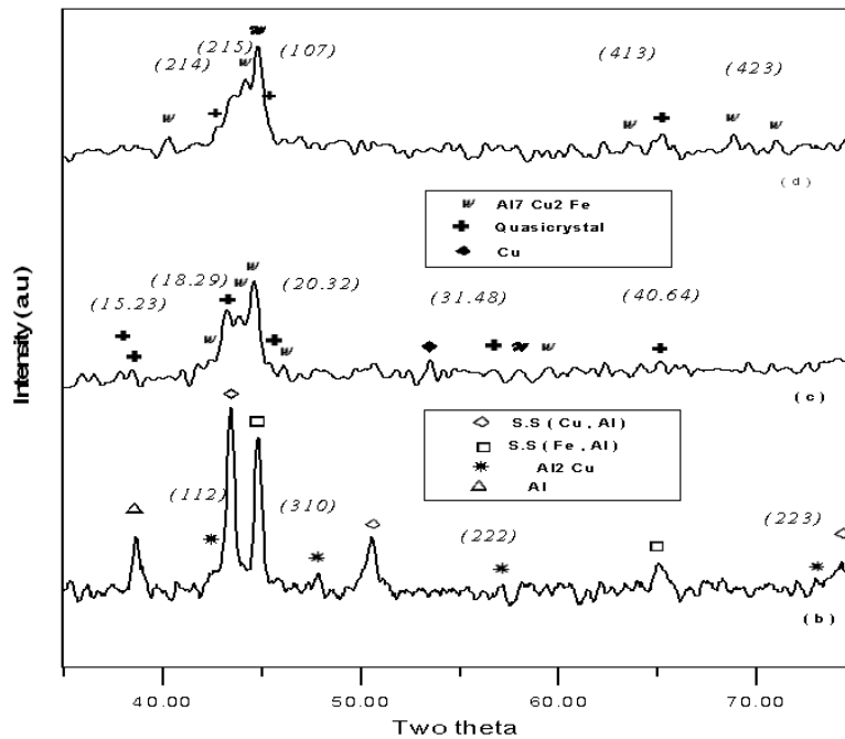
Fig. 8: XRD patterns of mechanically alloyed " Al_{62.5}Cu_{25}Fe_{12.5} " sample for: a) mixed elements (0 h), b) 10 hs, c) 20 hs, d) 30 hs.
