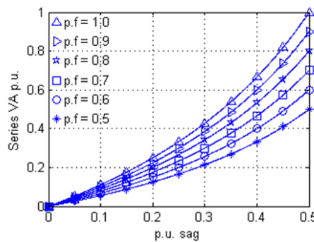
Fig. 4: VA loading of series inverter of UPQC for different power factor and p.u voltage sag values.
