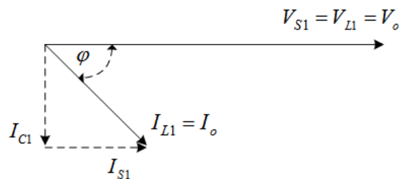
Fig. 2: Phasor diagram of shunt inverter of UPQC.
