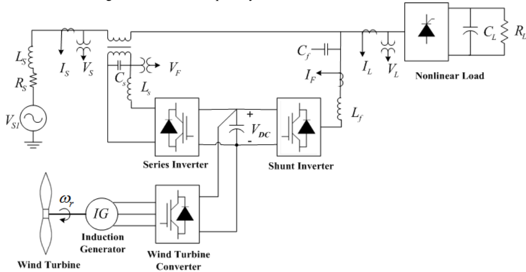
Fig. 1: Configuration of coupled operation of UPQC with WECS.
