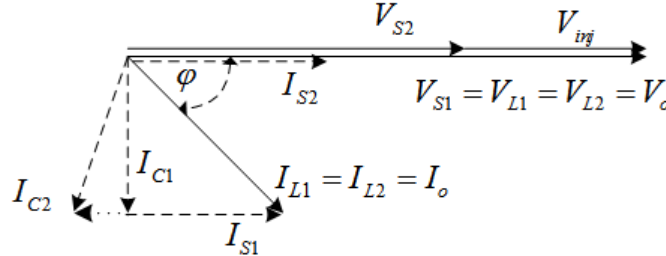
Fig. 3: Phasor diagram of shunt and series inverter of UPQC.
