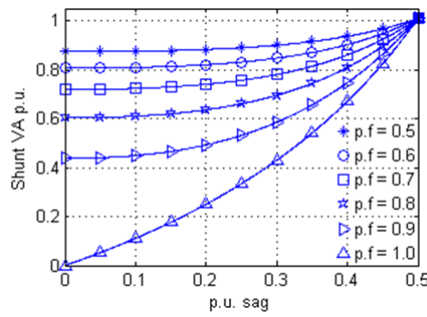
Fig. 5: VA loading of shunt inverter of UPQC for different power factor and p.u voltage sag values.
