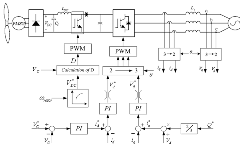
Fig. 3: Configuration and control system of proposed wind energy system. Natural frequency and damping ratio of boost converter are computed as follow (Ang and Oliva, 2005):
