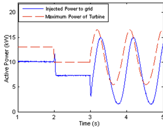
Fig. 9: Injected active power to grid, maximum mechanical power of turbine.
