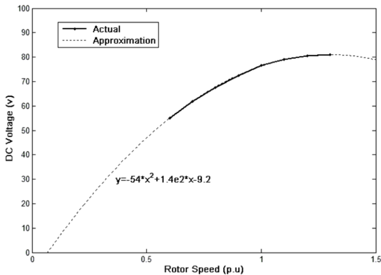
Fig. 5: DC voltage bus curve in term of optimum rotor speed obtained simulation and approximation.
