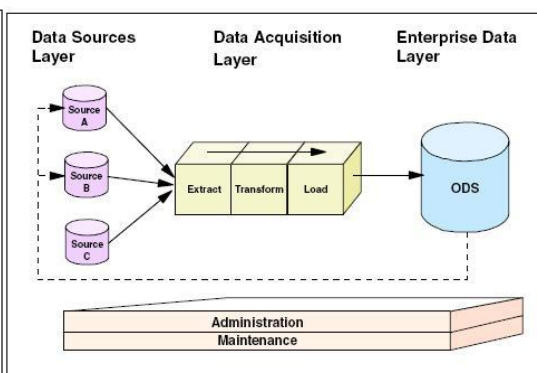
Fig. 2: General Architecture ODS.
