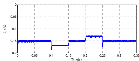
Fig. 7: Simulated output voltage and current of Negative output multiple lift-push-pull switched capacitor Luo converter with sudden load disturbances and regulatory responses (100Ω-90Ω V-100Ω -110Ω -100Ω)
