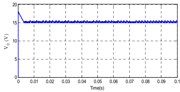
Fig. 4: Simulated start-up of the output voltage of Negative output multiple lift-push-pull switched capacitor Luo converter with set point 15V and nominal load 100Ω
