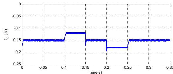
Fig. 6: Simulated output voltage and current of Negative output multiple lift-push-pull switched capacitor Luo converter with sudden line disturbances and servo responses (15V-12V-15V-18V-15V)
