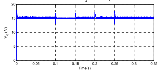
Fig. 6: Simulated output voltage and current of Negative output multiple lift-push-pull switched capacitor Luo converter with sudden line disturbances and servo responses (15V-12V-15V-18V-15V)
