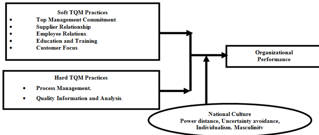
Fig. 1: Theoretical Framework.
