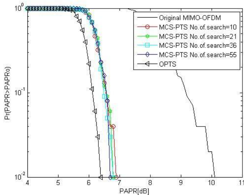
Fig. 5: CCDF of MCS technique for various searches when M = 8 , W = 2 .
