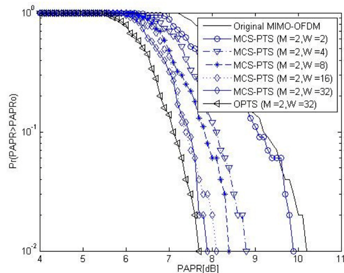
Fig. 4.1: Comparisons of MCS-PTS technique under different phase weight factors and M=2 subblock.
