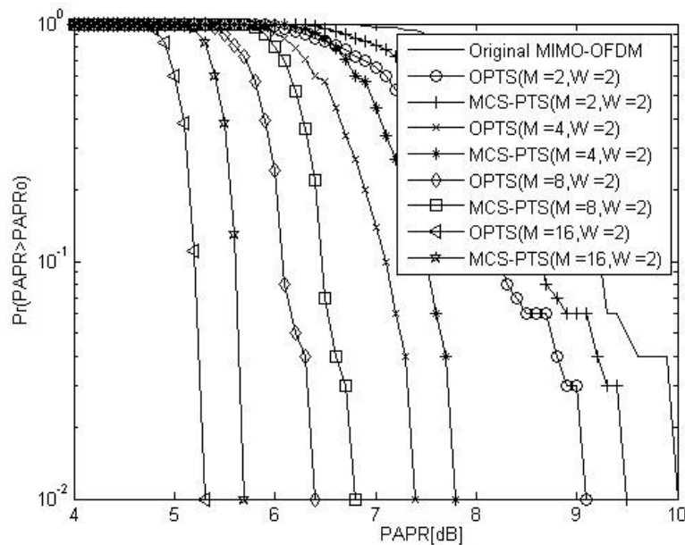
Fig. 3: CCDF of the PAPR with the PTS technique searched by MCS technique when N = 256 , M = 2, 4, 8 and 16 .
