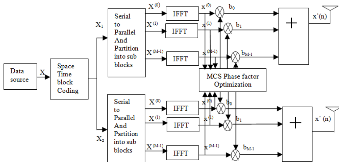
Fig. 1: Block Diagram of MCS-PTS model.
