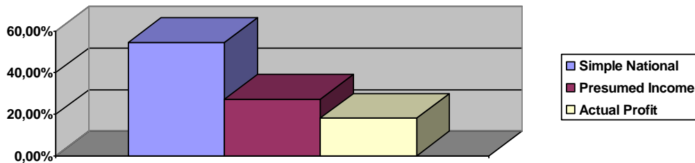
Fig. 3: Framework tax
