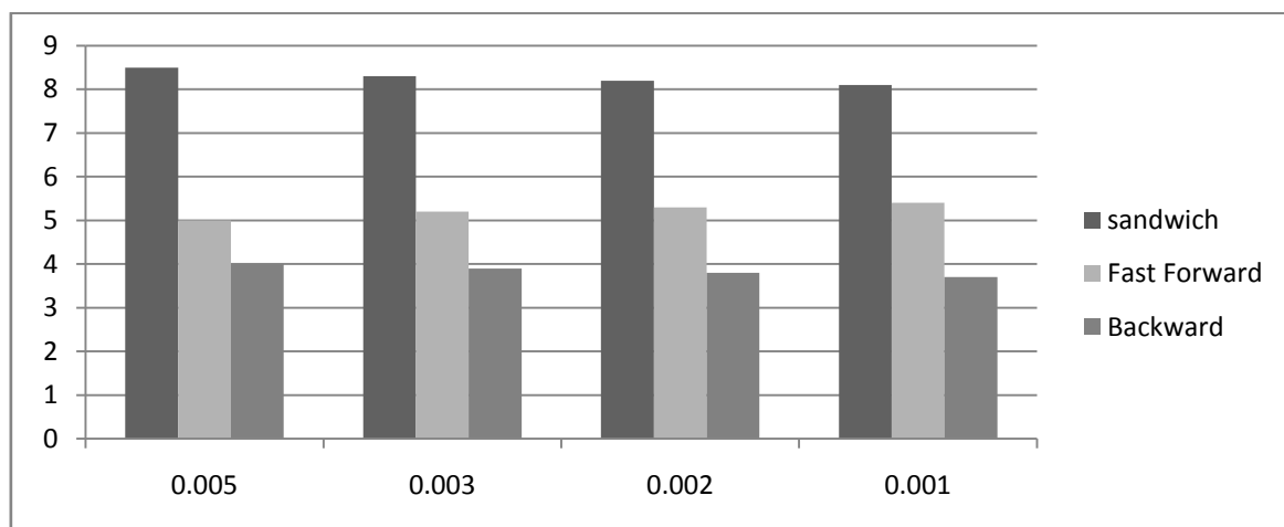
Fig. 1: Basic operation of three methods(X axis represents threshold values and Y axis represents number of basic operation that are needed).
